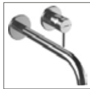
HANSAPUBLIC trim kit wall-mounted single-lever basin mixer, DN 15 suitable for installation unit HANSAVARIO* 5796 2171 chrome spout, Ø 26 mm, can be shortened from 300 to 235 mm projection: 300 mm
