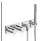
HANSALIVING trim kit installation set 13.2 thermostatic mixer, DN 15 (G1/2) suitable for HANSAMATRIX installation unit* 4487 0061 chrome suitable for HANSASIGNATUR, HANSALOFT, HANSADESIGNO, HANSALIGNA, HANSASTELA, HANSARONDA, shower set
