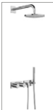
HANSALIVING trim kit installation set 11.3 thermostatic mixer, DN 15 (G1/2) suitable for HANSAMATRIX installation unit* 4487 0082 chrome suitable for HANSASIGNATUR, HANSALOFT, HANSADESIGNO, HANSALIGNA, HANSASTELA, HANSARONDA, with shower set, with HANSARAIN overhead shower, DN 15
