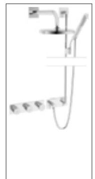
HANSALIVING trim kit installation set 14.1 thermostatic mixer, DN 15 (G1/2) suitable for HANSAMATRIX Tiptronik installation unit* 4487 0160 chrome suitable for HANSASIGNATUR, HANSALOFT, HANSADESIGNO, HANSALIGNA, HANSASTELA, HANSARONDA, wall bar set 1100 mm, with HANSARAIN overhead shower, DN 15
