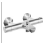
HANSAUNITA thermostatic bath faucet, DN 15 (G1/2) 5837 2101 chrome THERMO COOL - function projection: 180 mm
