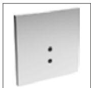
HANSAELECTRA trim kit with function unit concealed urinal trim kit, DN 15, mains supply suitable for HANSAELECTRA installation unit 0946 9172 chrome mains supply not included in delivery
