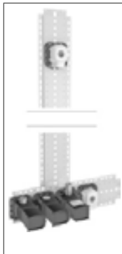
HANSAMATRIX Tiptronik installation unit set 14.0 thermostatic mixer, DN 15 (G1/2) 4486 0090 incl. power supply and connection cable, for two wall outlets
