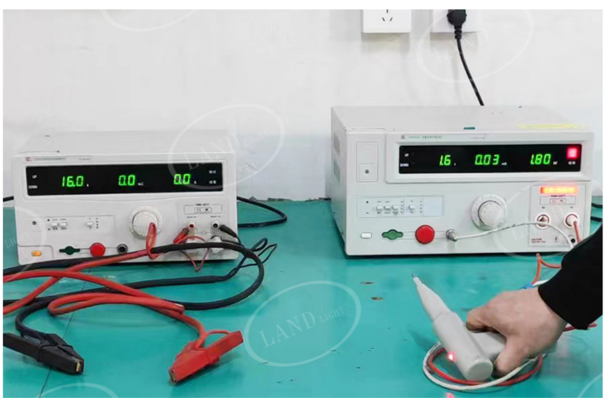
Ground high voltage test
