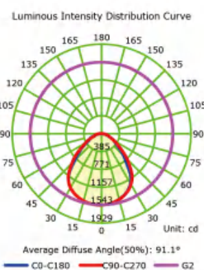
Prismatic diffuser Beam Angle : 91.1°
