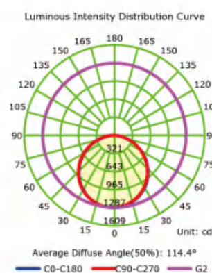
Opal diffuser Beam Angle : 114.4°
