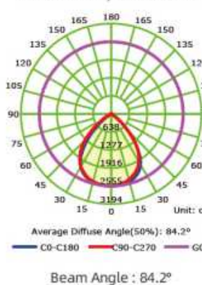
Luminous Intensity Distribution Curve
