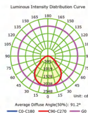
Prismatic diffuser Beam Angle : 91.2°
