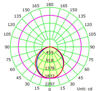
Opal Beam Angle
