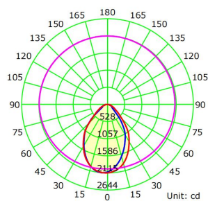
Microprism Beam Angle
