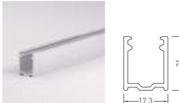
Aluminium Profile
