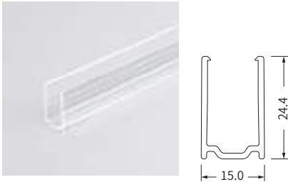
Dimension: 1000(±5)x15.0x24.4mm
