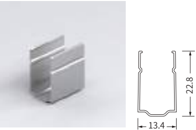
Dimension: 20x13.4x22.84mm
