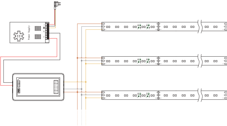
Installation Diagram
