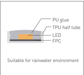
Drop PU glue with half tube
