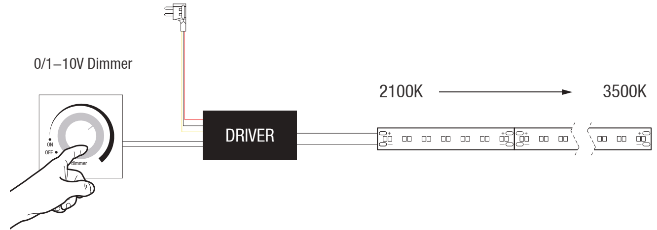
Wiring Diagram
