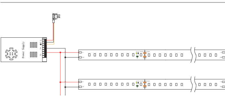
Installation Diagram
