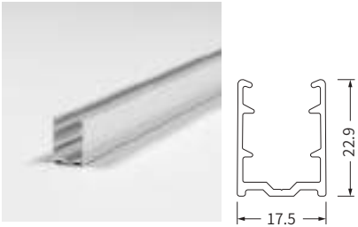
Dimension: 1000(±5)x17.5x22.9mm
