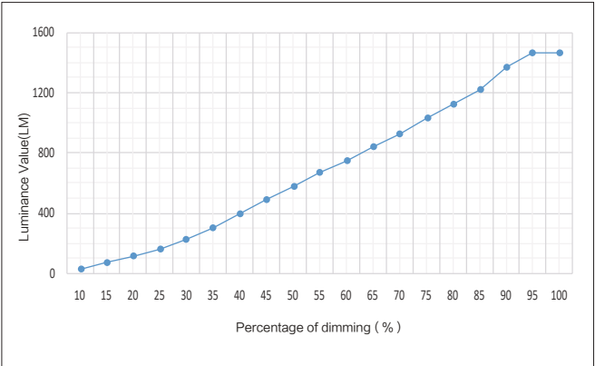
Luminance Curve
