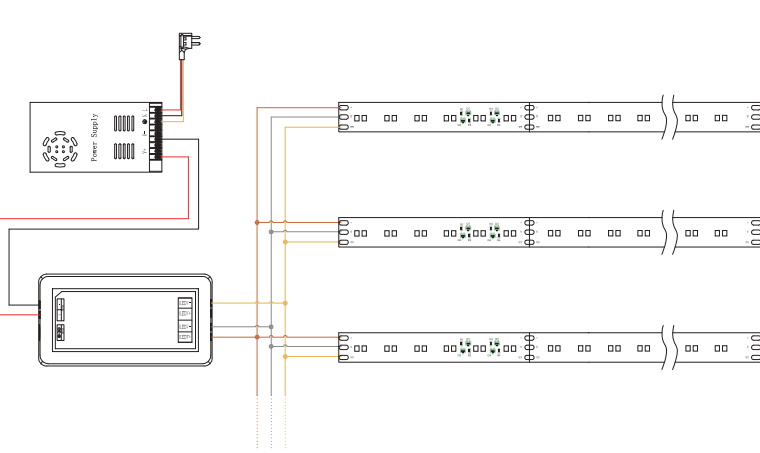
Installation Diagram
