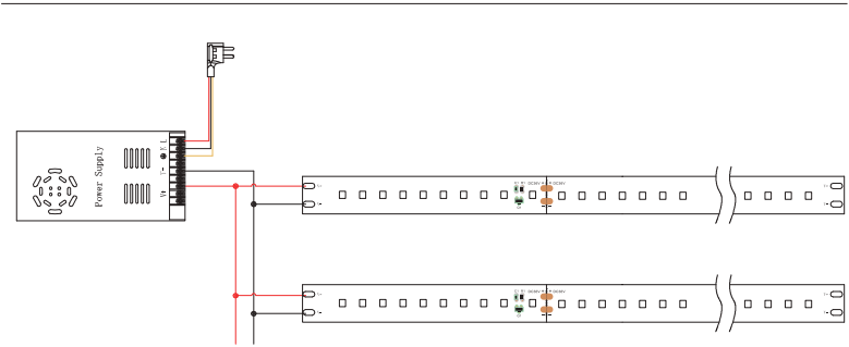
Installation Diagram
