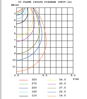
CD PLANE ISOLUX DIAGRAM (UNIT: lx)
