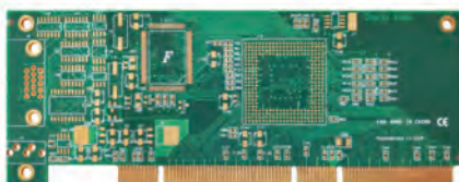
Video Card Board 4 layer, Gold Finger 显卡 金手指
