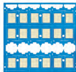
Cooling Backup Board Super -thin 0.4mm, 3W/(m·K)
