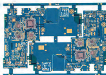
10L HDI 1+8+1 Finishing:OSP+ENIG HDI迭化工艺
