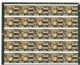
Bluetooth Wireless Modules Half-hole Process 蓝牙模块 半孔制程
