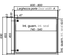
Vista frontale cassa Front box view 600-800
