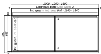
Vista frontale cassa Front box view 1000 - 1200 - 1600
