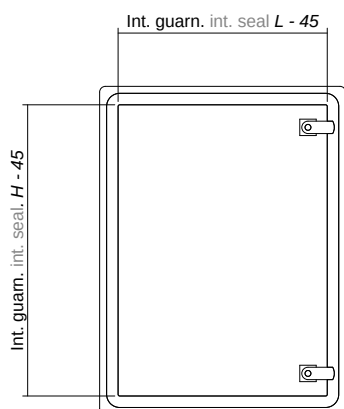
Vista interno porta Internal door view
