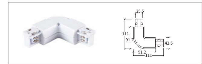
H-01 L型连接器-右 L-Connector-R
