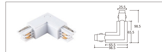
H-04 L型连接器-左 L-Connector-L
