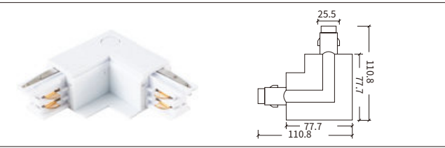
H-05 L型连接器-左 L-Connector-L
