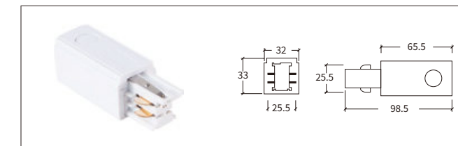
H-04 电源连接器-右 Feeder-R
