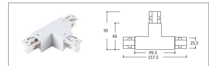
H-02 三向连接器-右 T-Connector-R
