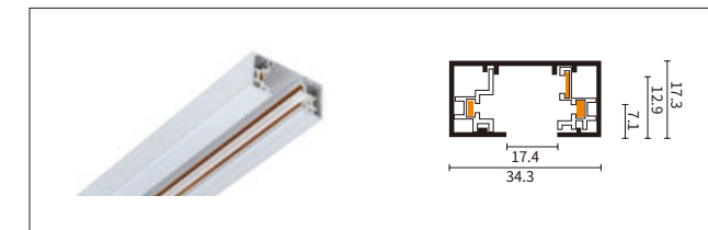
3线A 型美规导轨条 Three Line ASA Track
