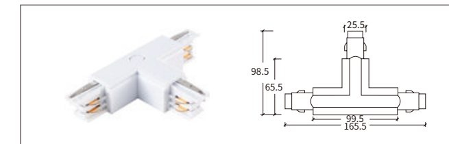
H-04 三向连接器-右 T-Connector-R
