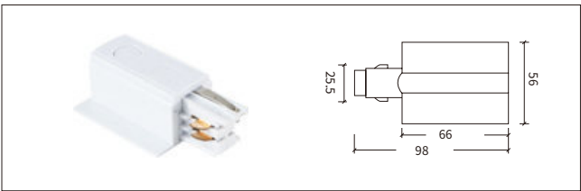
H-05 电源连接器-右 Feeder-R
