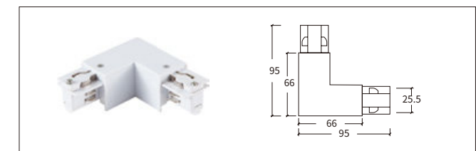
H-02 L型连接器-右 L-Connector-R
