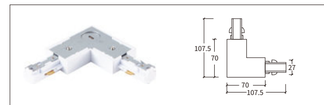
3线A L型连接器-左 L-Connector-L
