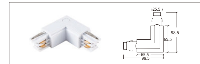
H-04 L型连接器-右 L-Connector-R
