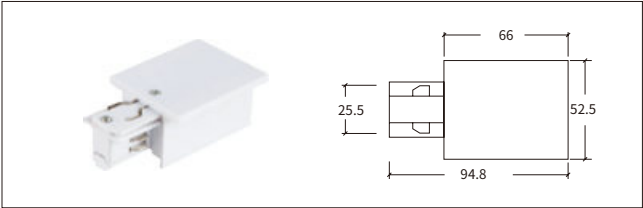
H-03 电源连接器-右 Feeder-R
