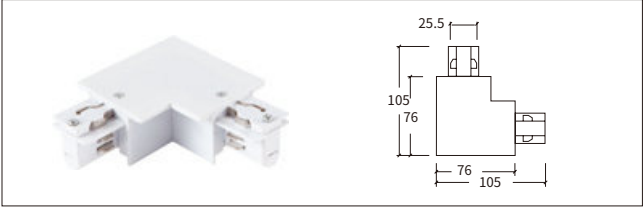
H-03 L型连接器-右 L-Connector-R
