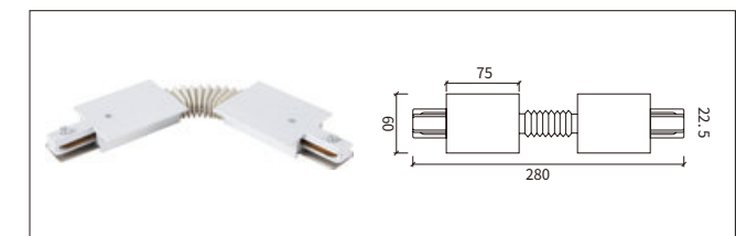
2 线嵌入式多角度连接器(软接 ) Flexible Connector
