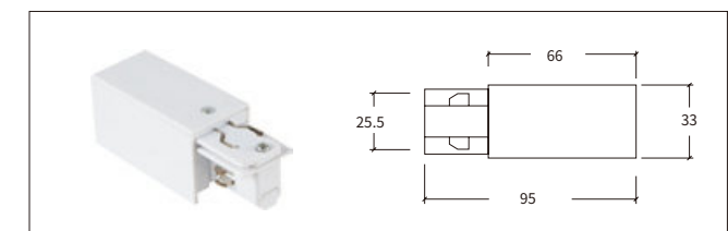
H-02 电源连接器-右 Feeder-R
