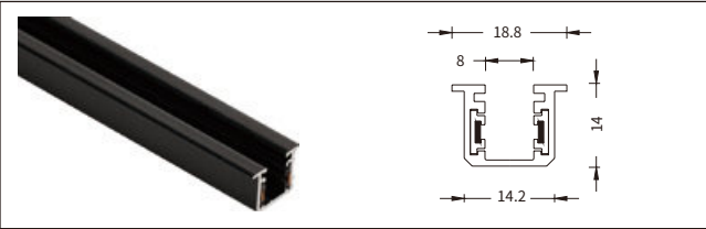
NO: YND-MINI-2-RE 嵌入式迷你导轨
