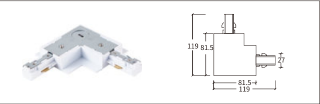
3线A嵌入式 L型连接器-右 L-Connector-R
