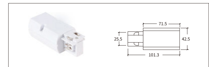
H-01 电源连接器-右 Feeder-R
