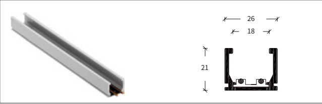
2 线低压导轨 (底部取电)
