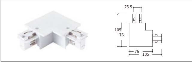
H-03 L型连接器-左 L-Connector-L
