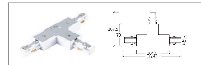
3线A 三向连接器-右 T-Connector-R
