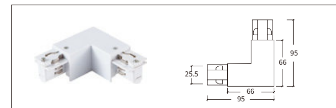
H-02 L型连接器-左 L-Connector-L
