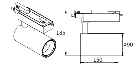
YND-GDT007-90 配电箱 Φ90 Driver Box Φ90
