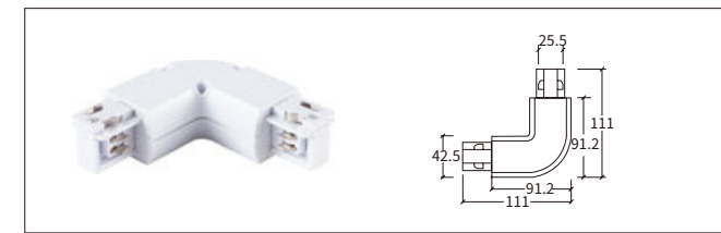
H-01 L型连接器-左 L-Connector-L
