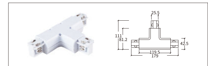
H-01 三向连接器-右 T-Connector-R
