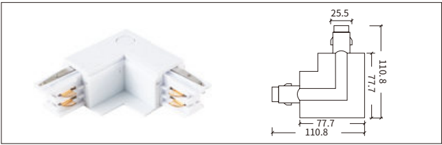
H-05 L型连接器-右 L-Connector-R
