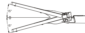
灯具水平安装, 可调角度为±15° Luminaire tilt adjustment, side entry: -15° to +15°
