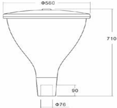
产品尺寸 Product Dimension
