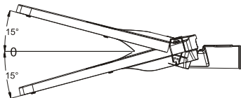
灯具水平安装, 可调角度为±15° Luminaire tilt adjustment, side entry: -15° to +15°
