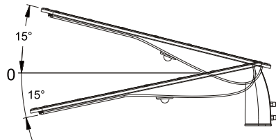
灯具水平安装，可调角度为±15° Luminaire tilt adjustment,side entry:-15°to+15°
