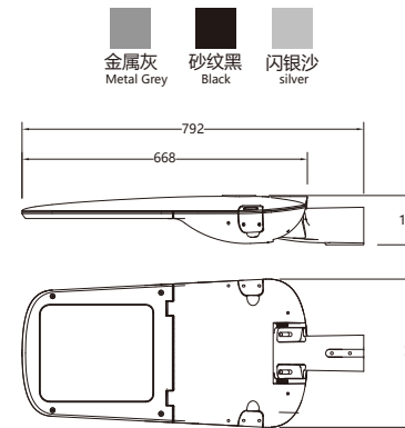
产品尺寸 Product Dimension
