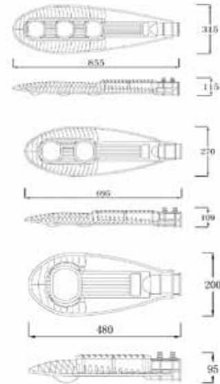
产品尺寸 Product Dimension
