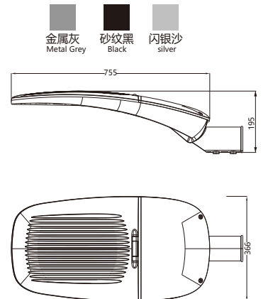
产品尺寸 Product Dimension
