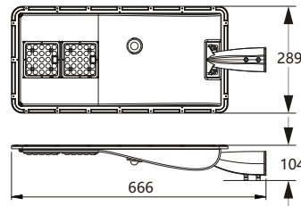
产品尺寸 Product Dimension
