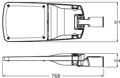
产品尺寸 Product Dimension
