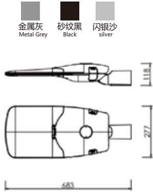
产品尺寸 Product Dimension
