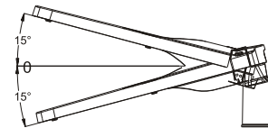
灯具竖直安装, 可调角度为0-15° Luminaire tilt adjustment, post top: 0° to +15°
