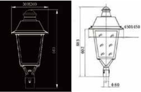
small size medium size 产品尺寸 Product Dimension
