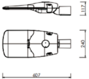
产品尺寸 Product Dimension
