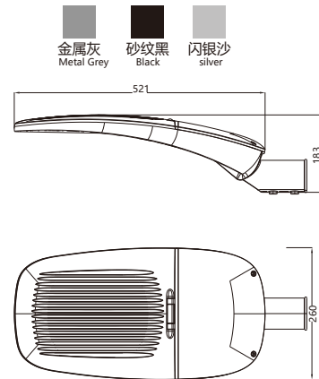
产品尺寸 Product Dimension
