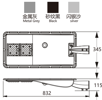
产品尺寸 Product Dimension
