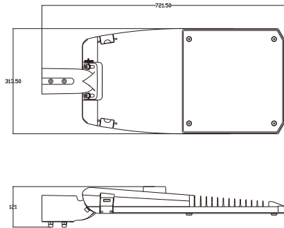
产品尺寸 Product Dimension
