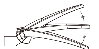
灯具水平安装, 可调角度为-20°~20° Luminaire tilt adjustment, side entry: -20° to +20°
