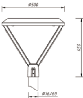
产品尺寸 Product Dimension
