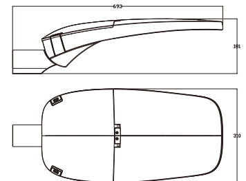
产品尺寸 Product Dimension
