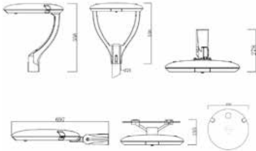
产品尺寸 Product Dimension
