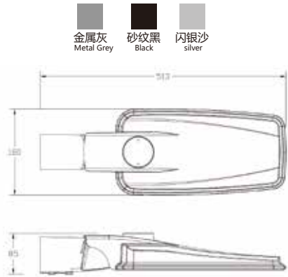
产品尺寸 Product Dimension
