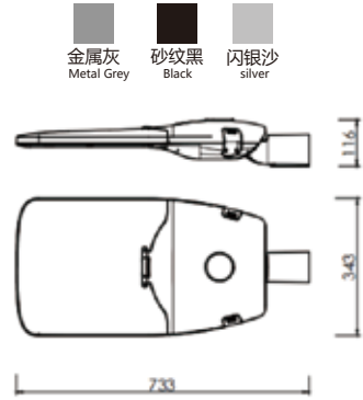
产品尺寸 Product Dimension
