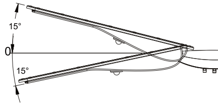
灯具垂直安装, 可调角度为0-15° Luminaire tilt adjustment, post top: 0° to +15°
