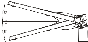
灯具垂直安装, 可调角度为0-15° Luminaire tilt adjustment, post top: 0° to +15°
