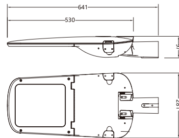
产品尺寸 Product Dimension
