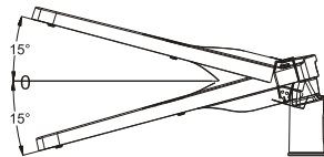
灯具竖直安装, 可调角度为0-15° Luminaire tilt adjustment, post top: 0° to +15°
