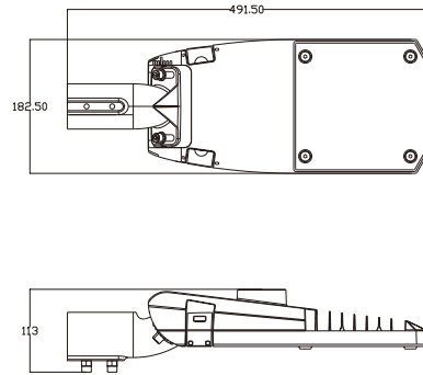
产品尺寸 Product Dimension
