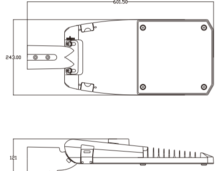
产品尺寸 Product Dimension
