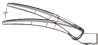
灯具水平安装, 可调角度为0-15° Luminaire tilt adjustment, side entry: 0° to +15°
