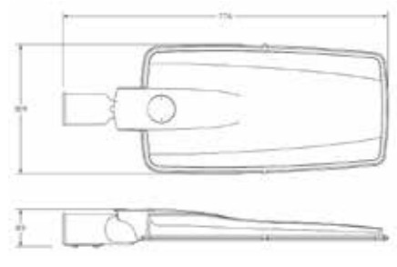
产品尺寸 Product Dimension
