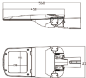
产品尺寸 Product Dimension
