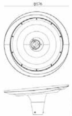
产品尺寸 Product Dimension
