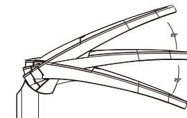
灯具竖直安装, 可调角度为-20°~20° Luminaire tilt adjustment, post top: -20° to +20°
