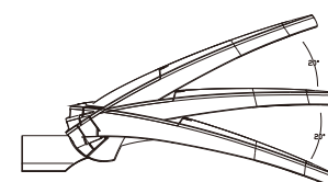
灯具水平安装, 可调角度为-20°~20° Luminaire tilt adjustment, side entry: -20° to +20°
