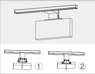
Mirror lamp + part A: Fixing on wall
