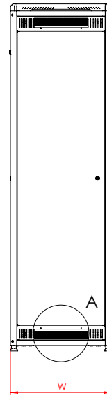
REAR VIEW
