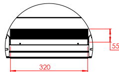
LOWER CHASSIS CABLE INPUT MODULE WITH BRUSH
