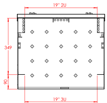
ASSEMBLY PROFILE
