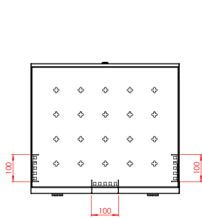
BOTTOM VIEW
