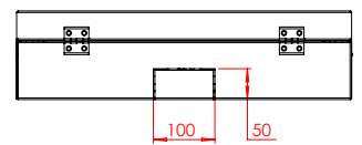
REAR VIEW
