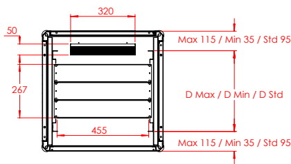
DEVICE ASSEMBLY DISTANCES CABLE INPUT SECTIONS
