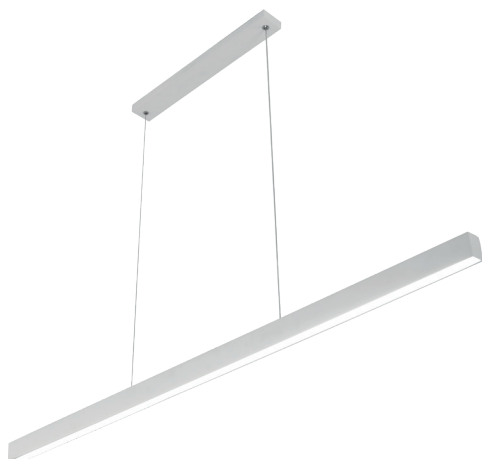
Lina BH16-09980 3 CCT 30W 3000lm White 220-240V CRI>80 IP20 Aluminium
