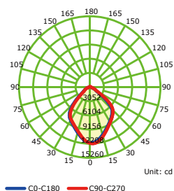
Luminous Intensity Distribution Curve (200W)
