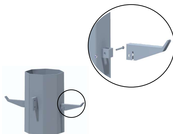
Removable rungs
