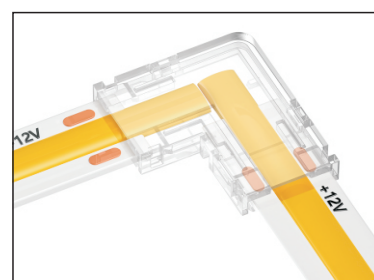
SS2L-8 8mm L shape
