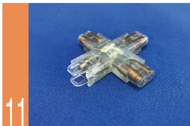
X Connector # BFXN 1xPower-in (Bottom) + 3xPower-out
