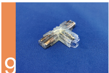
T Connector # BFTD 1xPower-in (Bottom) + 2xPower-out
