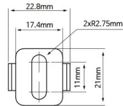
Mounting hole pattern
