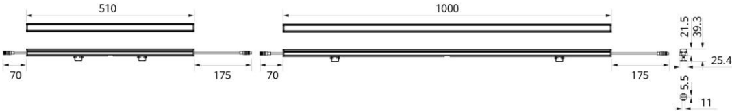
Adjustable Bracket Type
