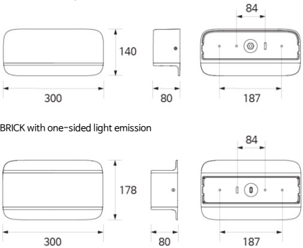
BRICK with two-sided light emission
