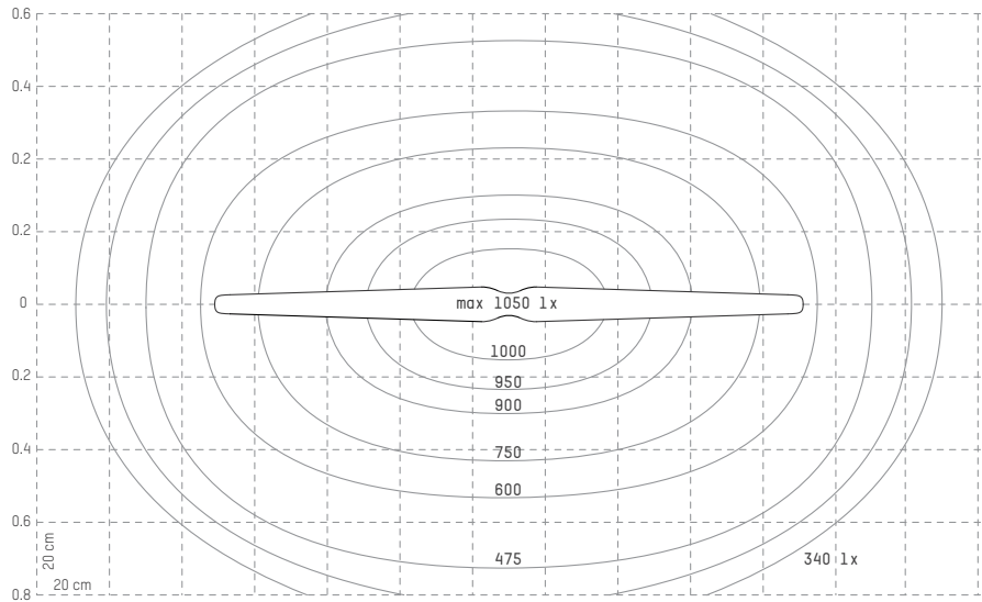
Swan Pendant 500mA lx measured 1.0 m on the table
