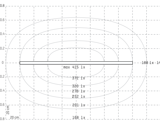
Led 120 1600 mm pendant lx / measured 1.0 m on the table
