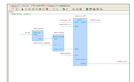
FBD – Functional block Diagram
