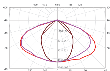
C plane light distribution curve
