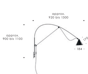
AYNO wall L wall / wand
