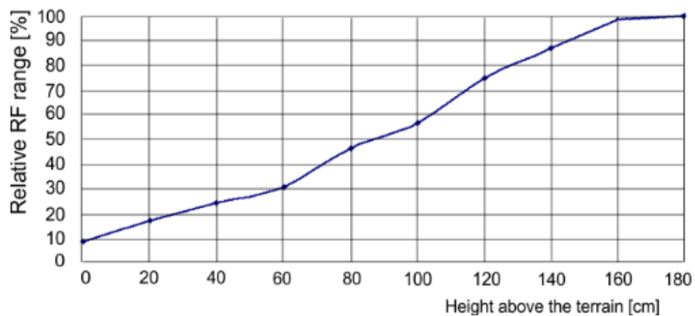
Diagram 4: TR-72DA relative RF range vs. antenna height above the ground, 868 MHz and 916 MHz bands.
