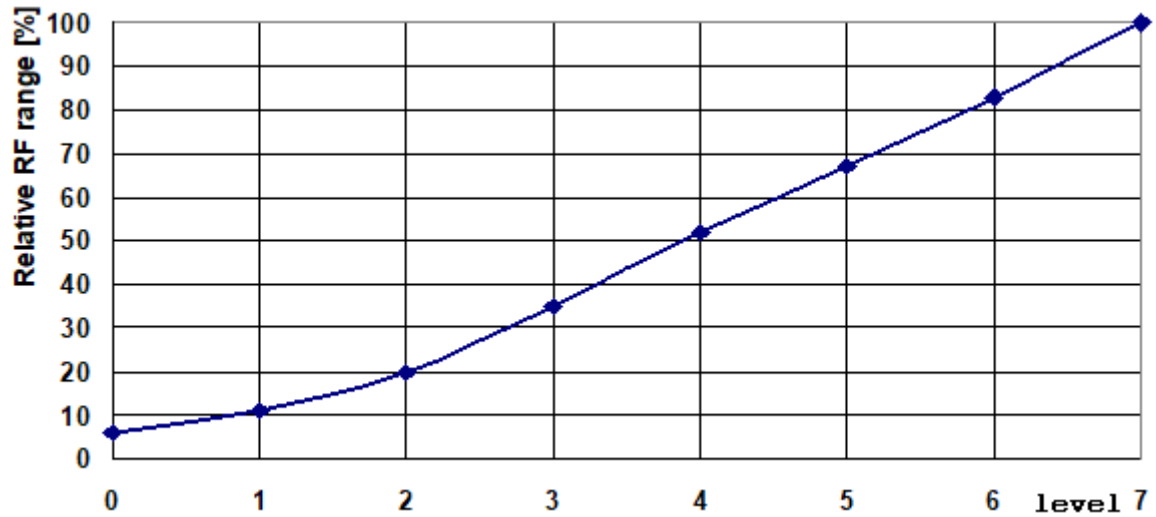
Diagram 2: Relative RF range vs. level in the setRFpower(level) function. TR-72D(A), 868 MHz and 916 MHz bands.
