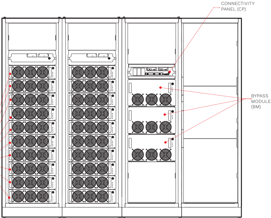
M2S 1000-1250 PCO without switches, up to 1000 or 1250 kW (front)
