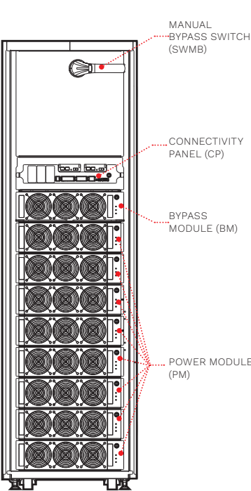
MP2 500 PCM with manual bypass up to 500 kW (front)
