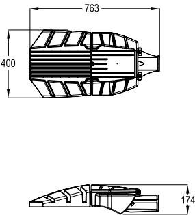
TRIMAX R0 - Side Entry (without LCU)
