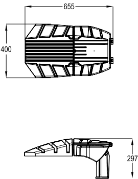
TRIMAX R0 - Post Top (without LCU)
