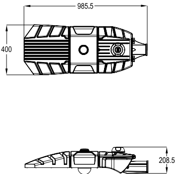
TRIMAX R3 - Post Top
