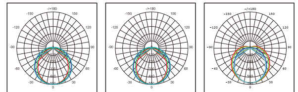
VE106GE02 Photometric VE112GE02 Photometric VE115GE02 Photometric
