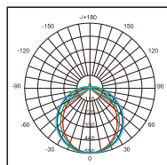
VE112GI Photometric
