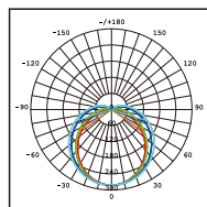
V3118D-LM Photometric
