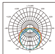
VE115GI Photometric
