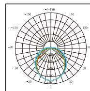
V3236BS-LM Photometric
