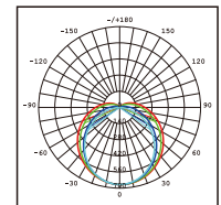
VE112GB-UL Photometric
