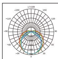
V5135B-LM Photometric
