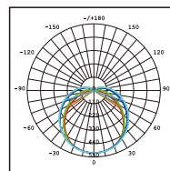
V3136D-LM Photometric
