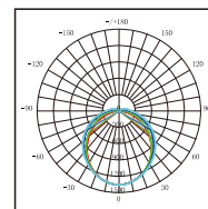
V3236D-LM Photometric
