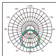
VE115GM Photometric
