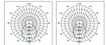
VE112DC 30W Photometric VE112DC 36W Photometric
