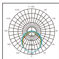
V3236G-LM Photometric
