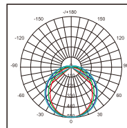
VE106GB Photometric
