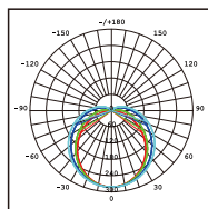
V3118BS-LM Photometric
