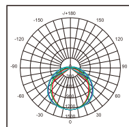
VE115GS Photometric
