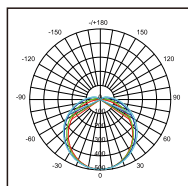
VE210FA Photometric
