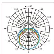
V5128C-LM Photometric
