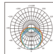
VE112SB Photometric
