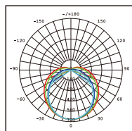
VE112GM Photometric
