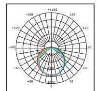
V3258D-LM Photometric
