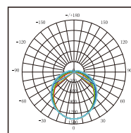
V5228B-LM Photometric
