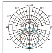
VC112E-16.5W Photometric
