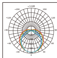
V3158D-LM Photometric
