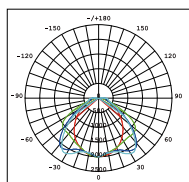
VE112SE Photometric
