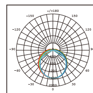
V5235B-LM Photometric
