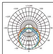
V3158BS-LM Photometric
