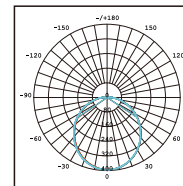
VC112E-21W Photometric
