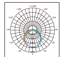
V3258D-LM Photometric
