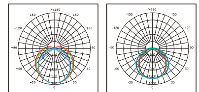
VE112GF Photometric
