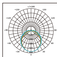
V5214B-LM Photometric
