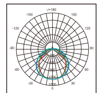
VE115SB Photometric
