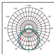
VE112GM02-M Photometric
