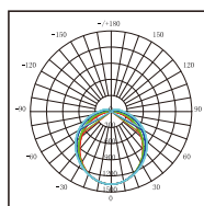
V5228C-LM Photometric
