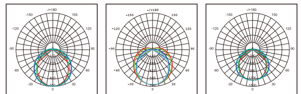
VE106GM02 Photometric VE112M02 Photometric VE115M02 Photometric
