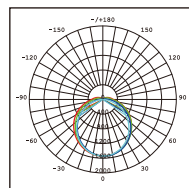
VE115N Photometric
