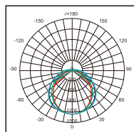
VE115GH Photometric
