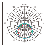
VE115DL-SU Photometric
