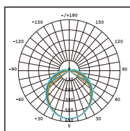
V5214C-LM Photometric
