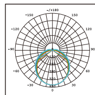
V3218BS-LM Photometric
