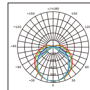
VE112X1 Photometric
