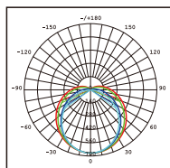
VE112GH Photometric
