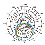
V3136BS-LM Photometric
