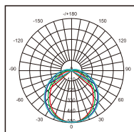
VE106GM Photometric
