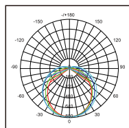
VE220FA Photometric
