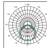
VE115GB Photometric
