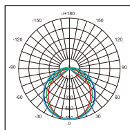
VE106DB02 Photometric
