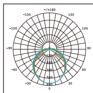
VE106N Photometric
