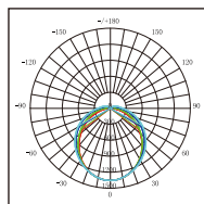
VE112N Photometric
