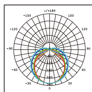
V5114B-LM Photometric
