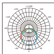
V3258G-LM Photometric
