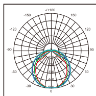
VE106DL-SU Photometric
