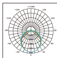
VLOE-206T Photometric
