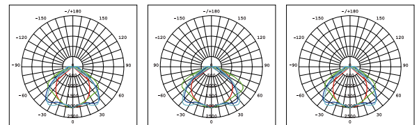
VE112SC Photometric
