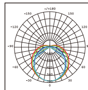
VE112GB Photometric
