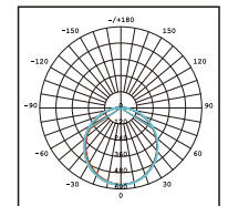
VC112E-22.5W Photometric
