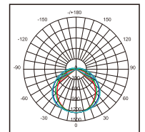
VE115X1 Photometric
