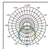
V3218D-LM Photometric
