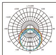
VE112GM02-MD Photometric
