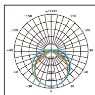
V5128B-LM Photometric
