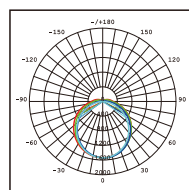
V3270G-LM Photometric
