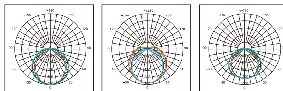
VE106DL-S Photometric VE112DL-S Photometric VE115DL-S Photometric
