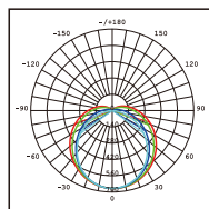
35W Photometric
