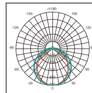
VE106X1 Photometric
