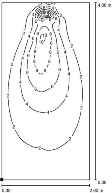
Dialux simulation
