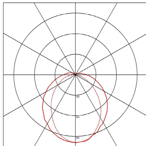
GalaLED LT model
