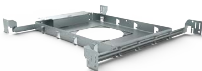
ACCH-12H-125 for EPIC135-4.5" Type: New construction plate
