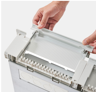
09 Removable cable entry for quick insertion of cables; one slider at top and bottom per module width
