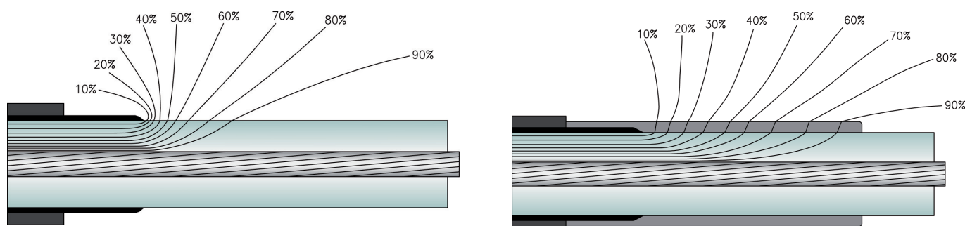
Fig. 2: Comparison of equipotential lines on cables without conductive layer and with refractive stress control.
