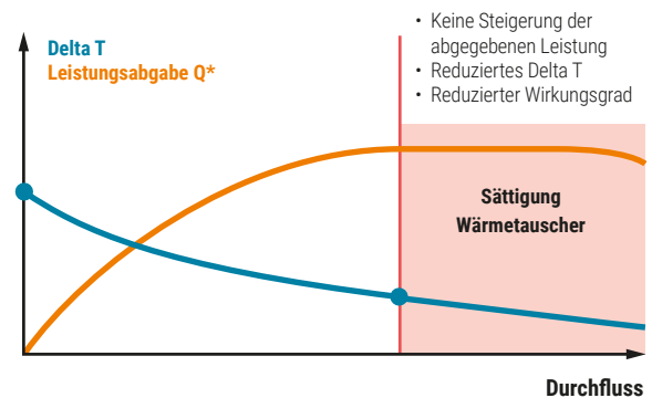
Abb. 51: Low-Delta-T-Syndrom
