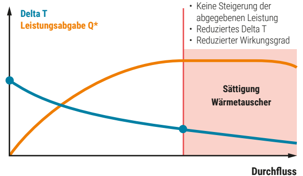
Abb. 106: Low-Delta-T-Syndrom
