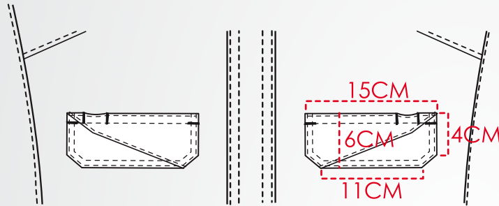
RIGHT POCKET Pen holder
