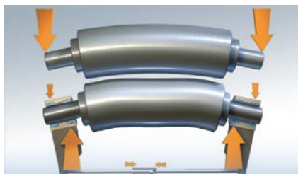
Standard single roll bending technology
