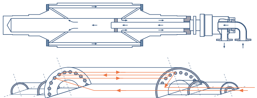
Peripheral bore of counter-roll with tripass system
