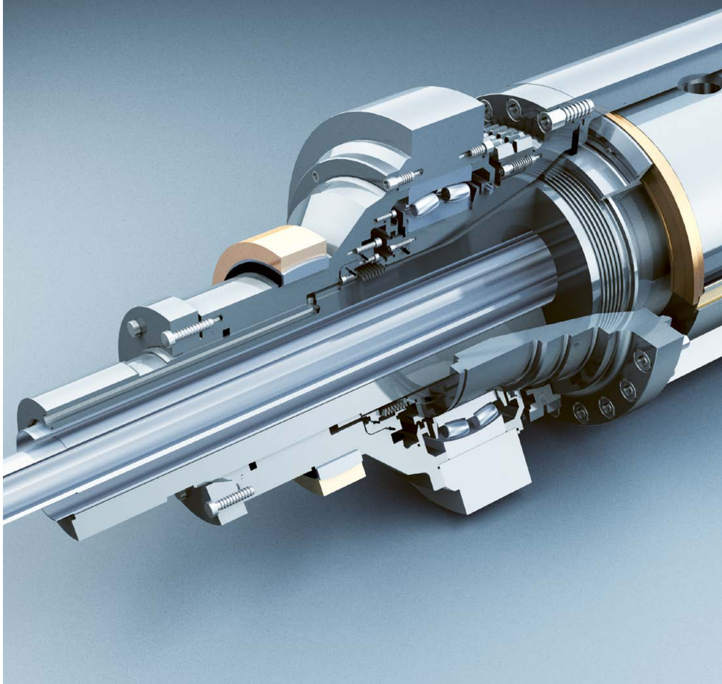
Inside of the Hot S-Roll
