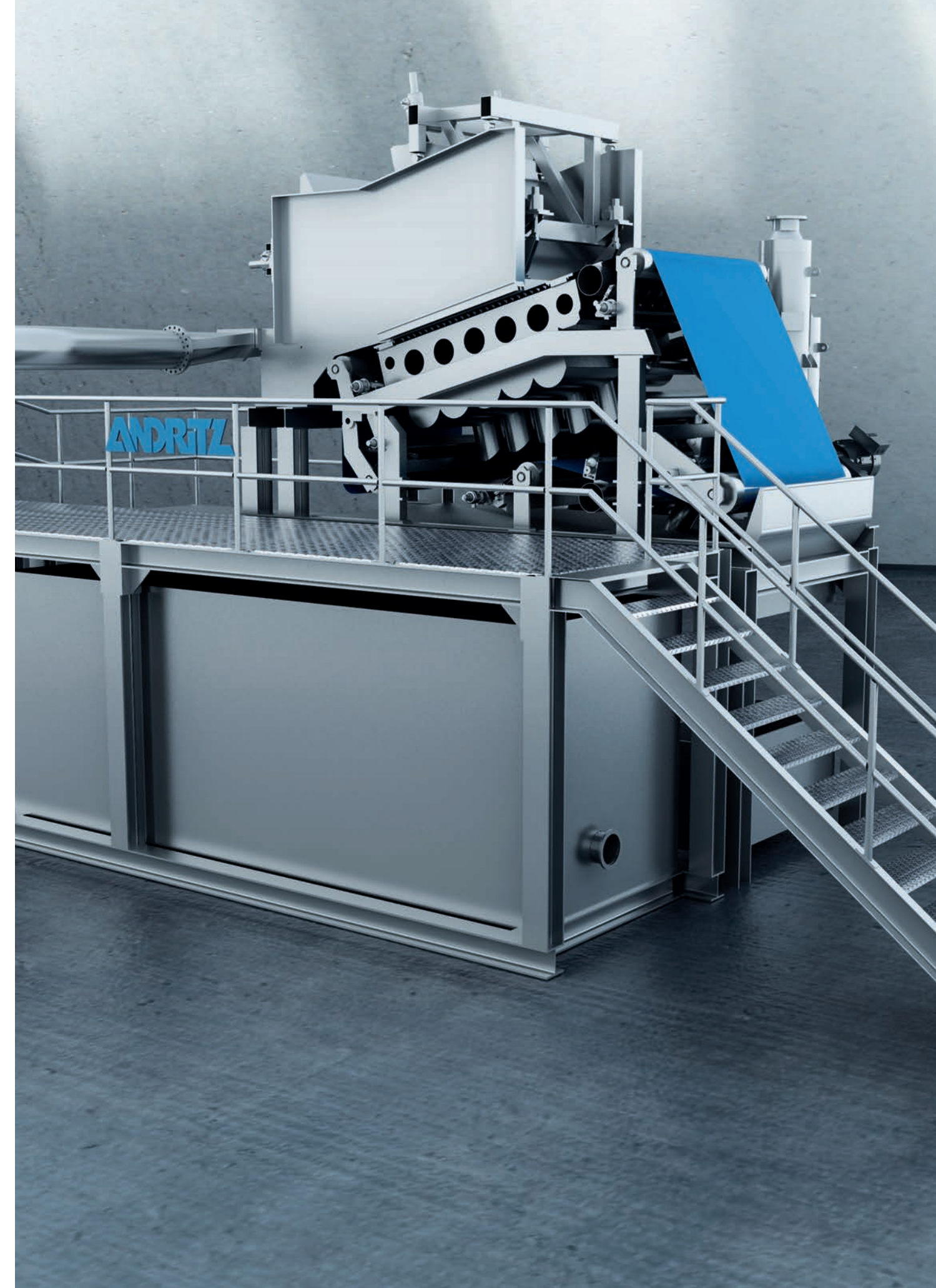
neXformer aXcess forming unit
