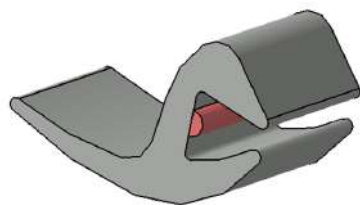
UVP 009 Universal profile with butyl, 18mm - 23m roll
