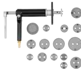
SGO Art. no 801016 Pneumatic brake caliper service set, 16-pcs
