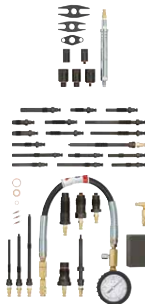
Art. no 818010 Master compression test set, 37-pcs
