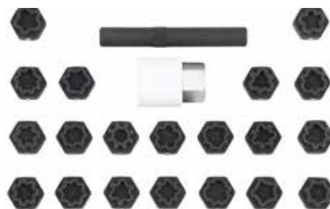
Art. no 829006 Wheel nut key set - Audi 22-pcs Audi set complete including 21mm adaptor with 1/2 "square drive. This kit is designed for the removal of locking bolts when the customer has forgotten to provide the adaptor with the car. This is happening very often when the vehicle is brought to maintenance and/or repair. Suitable for OEM T40073.
