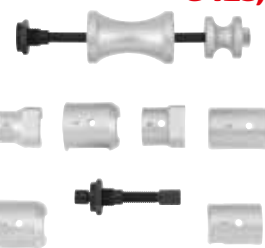
Art. no 812001 Wiper removal kit
