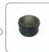
MIC1476 Lock ring 78 x 2,5 x 2,29 mm Application: G60/G85/GO110 OEM: 970 994 44 41
