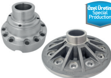
1368208 Diff. Half Housing 1pc + 1368527 Diff. Half Housing 1pc
