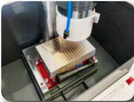
Piano magnetico a poli fitti Dense polarity magnetic chuck
