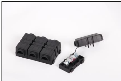
MidiType Fuse Holder (Product codes: FH1001)
