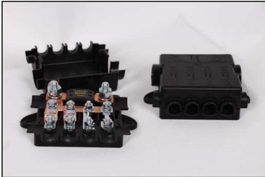
Combi Fuse Holder (product code: FH1005-A & FH1005-B)
