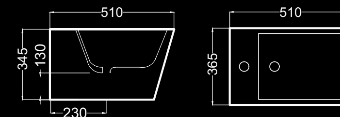
Bidet suspendido Wall-hung bidet Bidet suspendu 25 Kg
