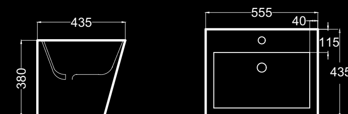
Lavabo mural Wall-hung basin Lavabo mural 31,7 Kg
