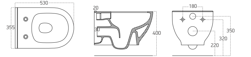
RIM ART WALL-HUNG CLOSET
