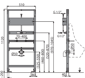
AS107S/1120 Mounting frame for urinal and sensor
