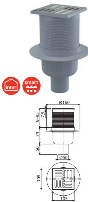
APV32 Floor drain 105×105/50 mm straight outlet, stainless steel grid, combined odour trap SMART
