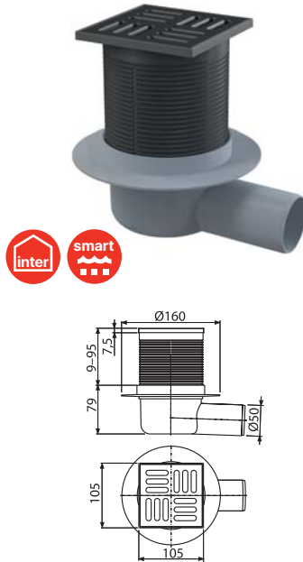
APV31BLACK new Floor drain 105×105/50 mm side outlet, stainless steel grid black-matt, combined odour trap SMART
