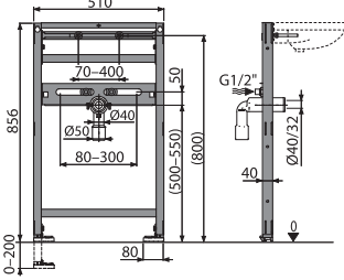
AS104/850 Mounting frame for wash-basin
