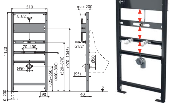
A107S/1120 Mounting frame for urinal and sensor
