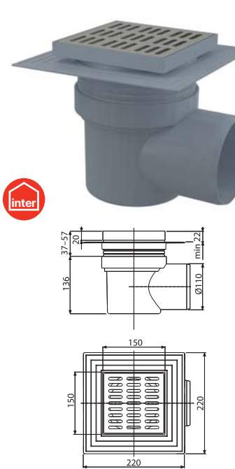
APV12 Floor drain 150×150/110 mm side outlet, stainless steel grid, collar-2nd level insulation, wet odour trap
