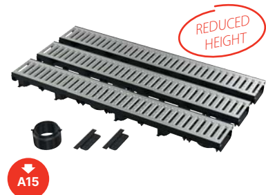
AVZ112-G102 Garage pack 3 m (2x end cap, 1x socket DN110)
