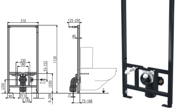
A113/1120 Mounting frame for wall-hung WC combi
