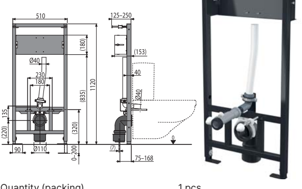
A114S/1120 Mounting frame for wall-hung WC and sensor
