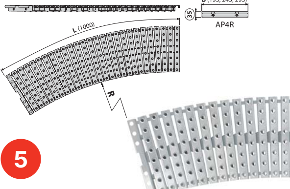
AP4R Swimming pool overflow radius grating with anti-slip surface
