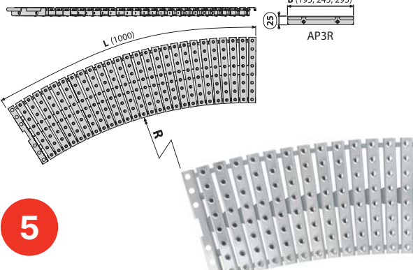
AP3R Swimming pool overflow radius grating with anti-slip surface
