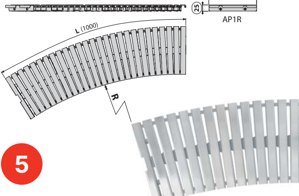
AP1R Swimming pool overflow radius grating without anti-slip surface
