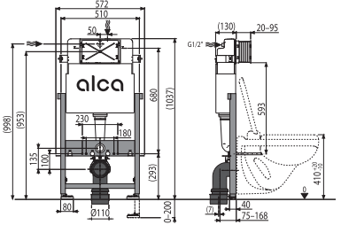
AS101 Sádromodul Pre-wall installation system for dry build up (plasterboard)
