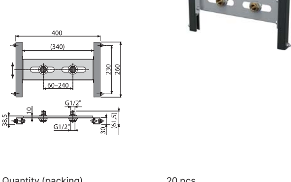
A117B Mounting frame for faucet in plaster-board structure
