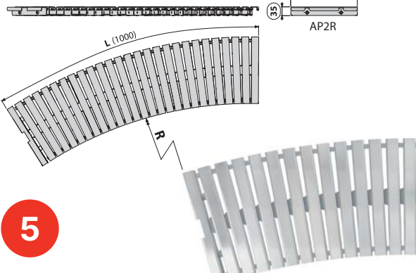
AP2R Swimming pool overflow radius grating without anti-slip surface
