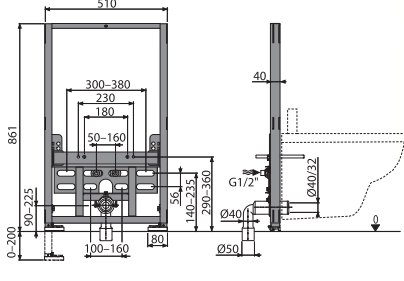
AS105/850 Mounting frame for bidet
