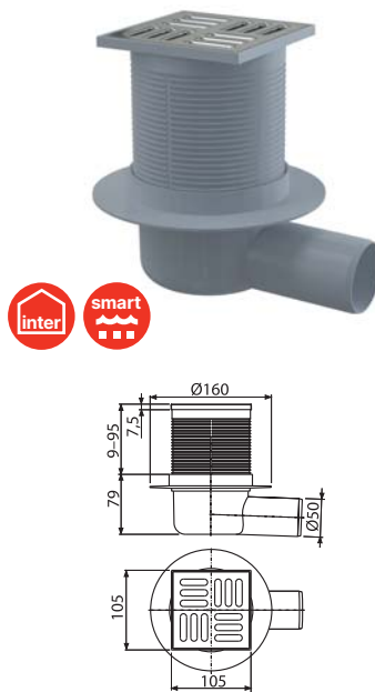
APV31 Floor drain 105×105/50 mm side outlet, stainless steel grid, combined odour trap SMART
