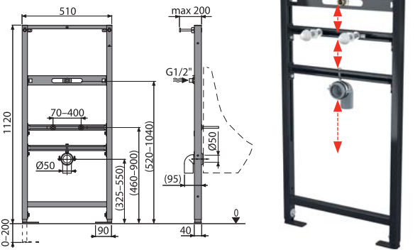
A107/1120 Mounting frame for urinal
