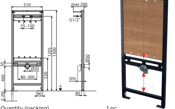
A108/1300 Mounting frame for waste sink and faucet
