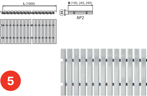
AP2 Swimming pool overflow grating without anti-slip surface
