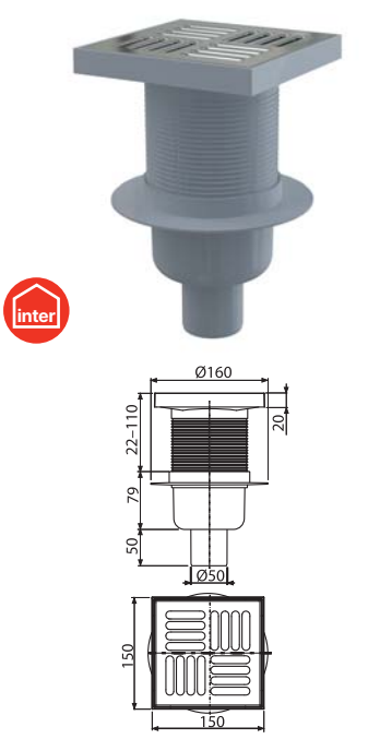
APV641I Floor drain 150×150/50 mm straight outlet, stainless steel grid, wet odour trap
