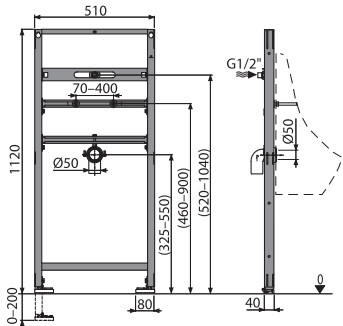
AS107/1120 Mounting frame for urinal
