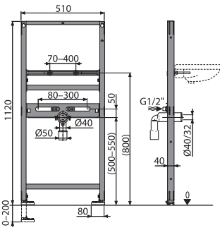
AS104/1120 Mounting frame for wash-basin
