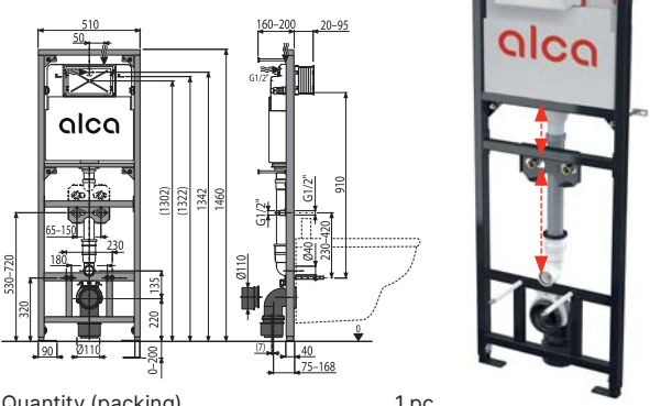
A108F/1500 Mounting frame with cistern for a waste sink with waste connection DN90/110 and faucet
