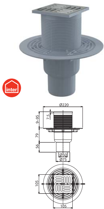
APV231I Floor drain 105×105/50/75 mm straight outlet, stainless steel grid, wet odour trap
