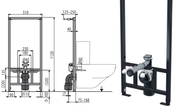
A114/1120 Mounting frame for wall-hung WC
