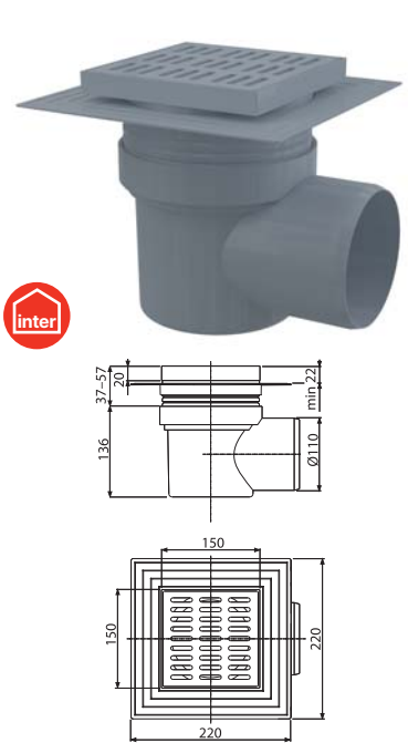
APV10 Floor drain 150×150/110 mm side outlet, grey grid, collar-2nd level insulation, wet odour trap
