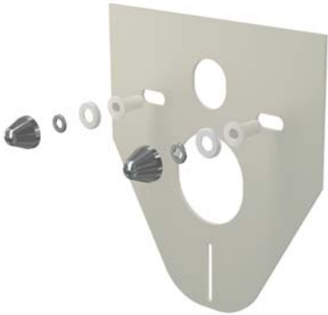
M910CR Noise insulation for wall-hung WC toilets and bidets with accessories including cover cap (chrome)
