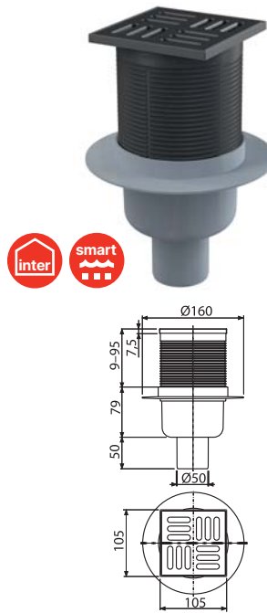
APV32BLACK new Floor drain 105×105/50 mm straight outlet, stainless steel grid black-matt, combined odour trap SMART
