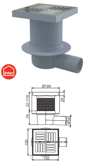
APV541I Floor drain 150×150/50 mm side outlet, stainless steel grid, wet odour trap
