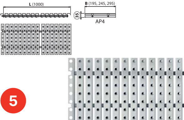
AP4 Swimming pool overflow grating with anti-slip surface
