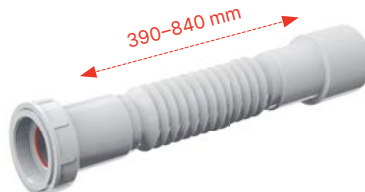
A793 Flexi pipe 6/4" with reduction to 5/4"×50/40 plastic
