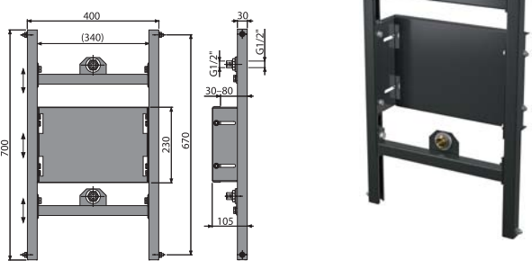
A117PB Mounting frame for built-in mixer in plaster-board structure
