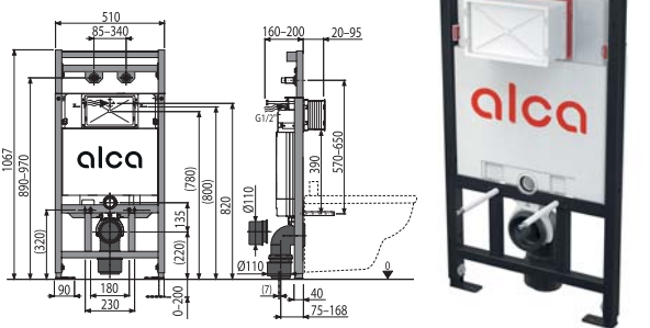
A108F/1100 Mounting frame with cistern for a waste sink with waste connection DN90/110 and faucet
