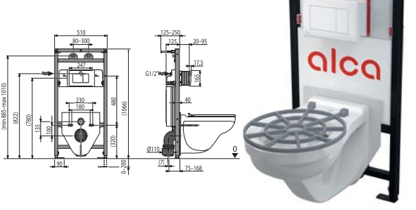
A108F 5:1 SET Set: mounting frame, waste sink inc. grid, insulation, flush plate
