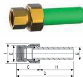
BOCCHETTONE FILETTATO FEMMINA saldatura a bicchiere con codoli in PP-RCT THREADED PIPE UNION FEMALE socket welding with PP-RCT shank
