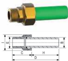
BOCCHETTONE FILETTATO MASCHIO saldatura a bicchiere con codoli in PP-RCT THREADED PIPE UNION MALE socket welding with PP-RCT shank
