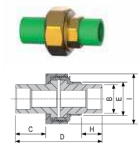
BOCCHETTONE a saldare femmina saldatura a bicchiere con codoli in PP-RCT PIPE UNION to weld female socket welding with PP-RCT shank
