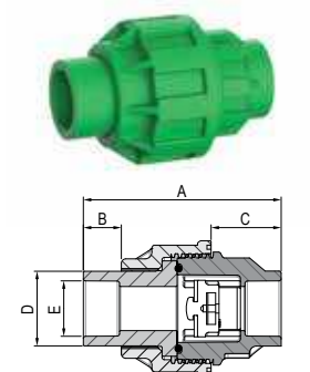
BOCCHETTONE IN PP-RCT saldatura a bicchiere PP-RCT PIPE UNION socket welding
