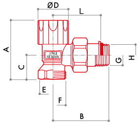
DS 32 Angle regulating lockshield. Connection for copper and plastic pipe.
