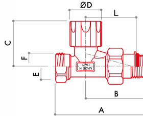
DD 31 Straight regulating lockshield. Connection for copper and plastic pipe.
