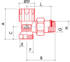
DS 39 Angle regulating lockshield. Connection for copper and plastic pipe.
