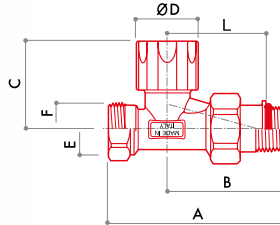
DD 38 Straight regulating lockshield. Connection for copper and plastic pipe.
