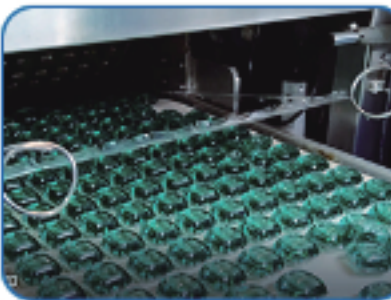
3. Sealing & cutting
