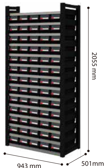
RCH-313 943W x 468D x 2055H mm
