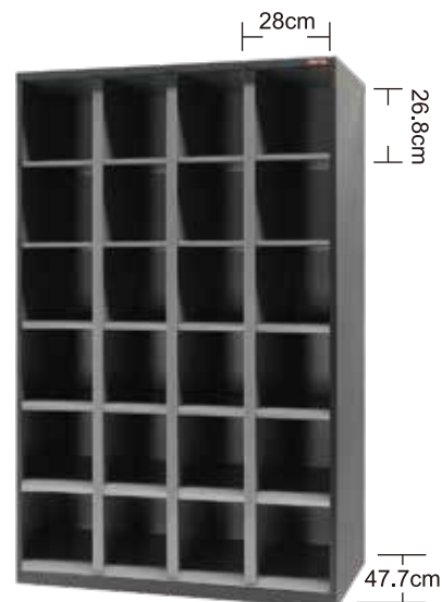
FCO-424 1182W x 510D x 1800H mm
