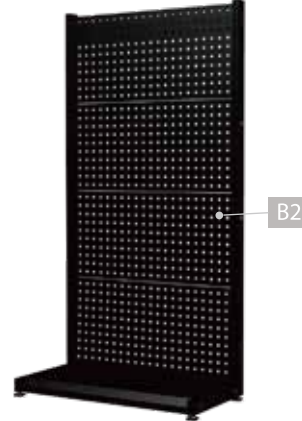
DS-1400 914W x 452D x 1708H mm
