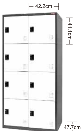
FC-208 FC-208K (key lock) 900W x 510D x 1800H mm
