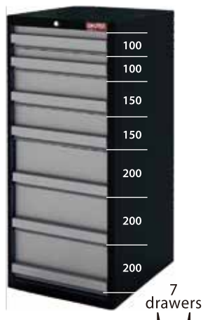
HDC-1271 548W x 608D x 1200H mm
