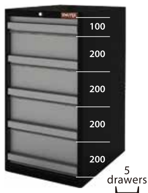
HDC-1051 548W x 608D x 1000H mm
