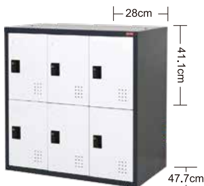
FC9-306 FC9-306K (key lock) 900W x 510D x 895H mm
