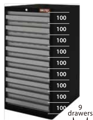
HDC-1091 548W x 608D x 1000H mm
