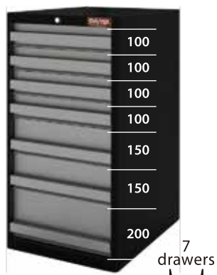
HDC-1072 548W x 608D x 1000H mm
