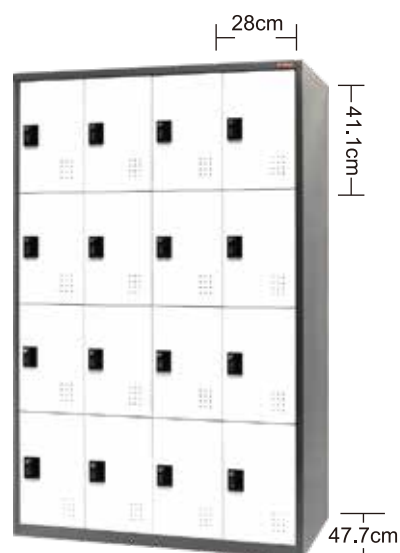
FC-416 FC-416K (key lock) 1182W x 510D x 1800H mm
