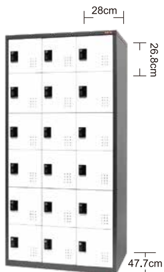
FC-318 FC-318K (key lock) 900W x 510D x 1800H mm
