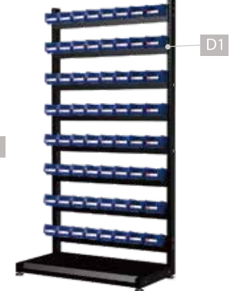
DS-8945+H1088 914W x 452D x 1708H mm
