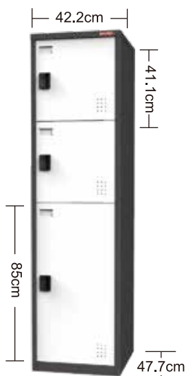
FC-M103 FC-M103K (key lock) 477W x 510D x 1800H mm
