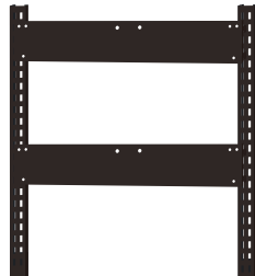
CW62 674W x 25D x 632H mm Optional: FO-604x2
