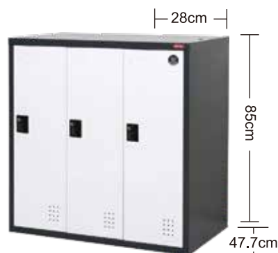
FC9-303 FC9-303K (key lock) 900W x 510D x 895H mm
