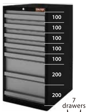
HDC-1071 548W x 608D x 1000H mm
