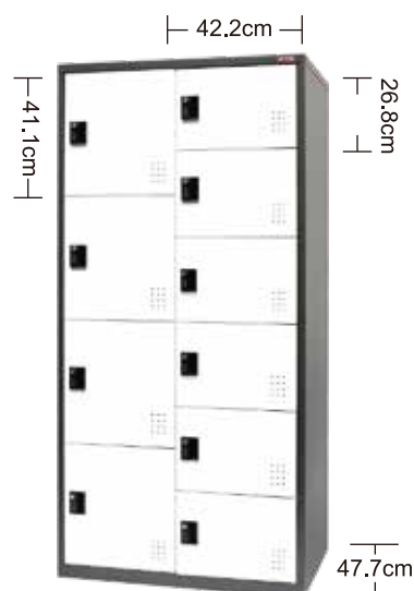
FC-M210 FC-M210K (key lock) 900W x 510D x 1800H mm
