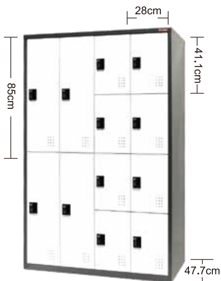
FC-M412 FC-M412K (key lock) 1182W x 510D x 1800H mm
