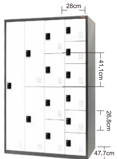
FC-M413 FC-M413K (key lock) 1182W x 510D x 1800H mm
