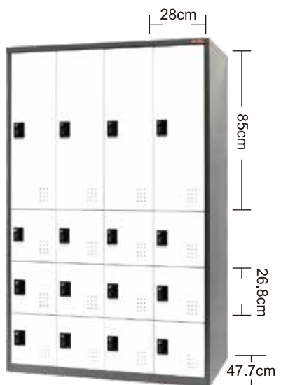
FC-M416 FC-M416K (key lock) 1182W x 510D x 1800H mm
