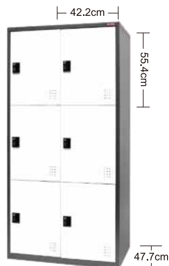
FC-206 FC-206K (key lock) 900W x 510D x 1800H mm
