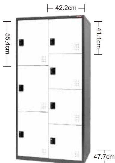
FC-M207 FC-M207K (key lock) 900W x 510D x 1800H mm
