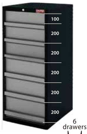
HDC-1261 HDC-1261T 548W x 608D x 1200H mm
