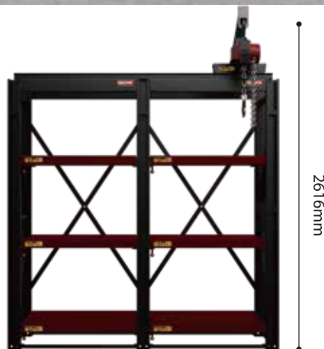
TM-2061C 2110W x 876D x 2616H mm (Dimensions include crane)
