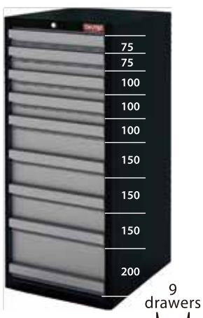
HDC-1291 548W x 608D x 1200H mm
