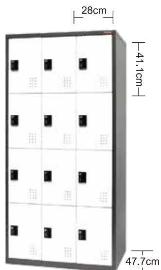
FC-312 FC-312K (key lock) 900W x 510D x 1800H mm
